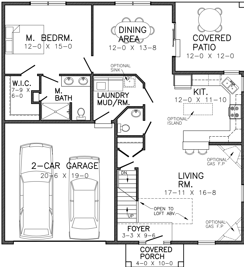
FIRST FLOOR PLAN 1211 SQ.FT.
