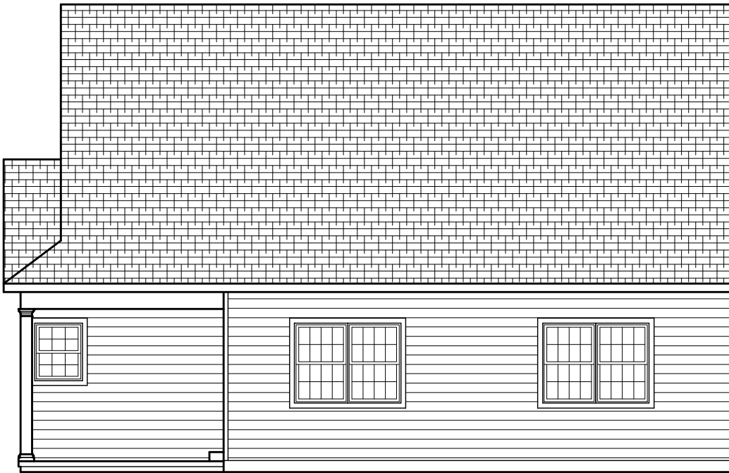
REAR ELEVATION
