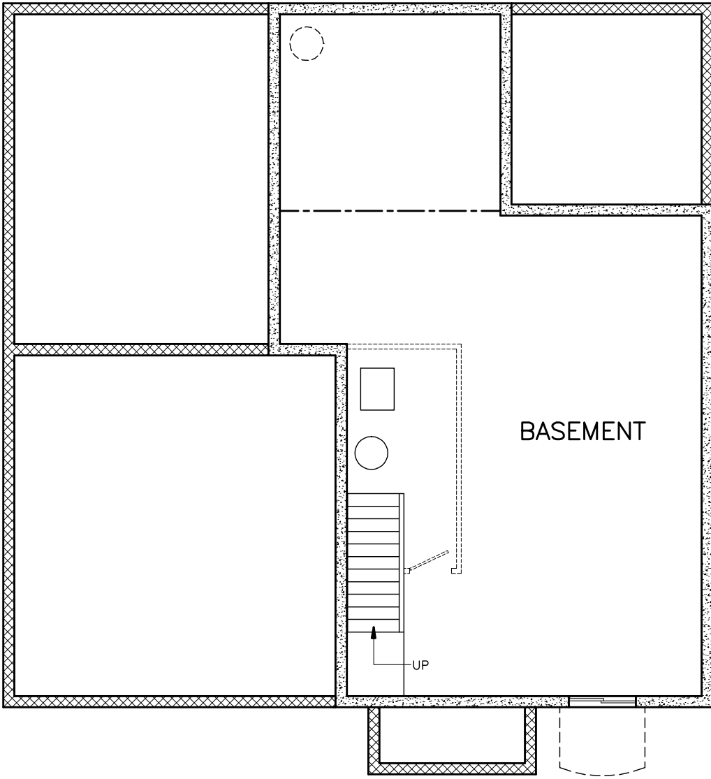
FOUNDATION PLAN
