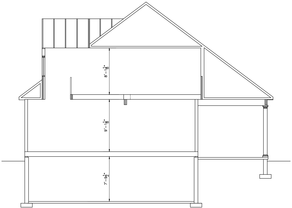
CROSS SECTION
